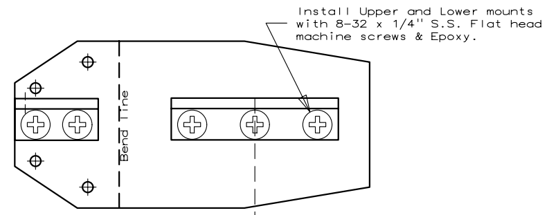
Assembly View (shown unbent for ref. only)
